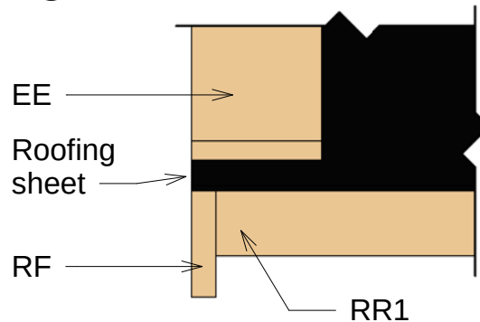
③ Roof Reinforcement
